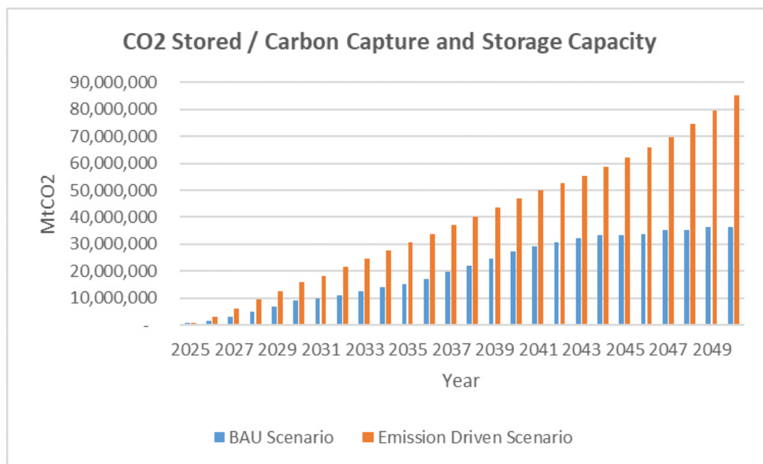
Figure 28: CO 2 stored and CCS Capacity
