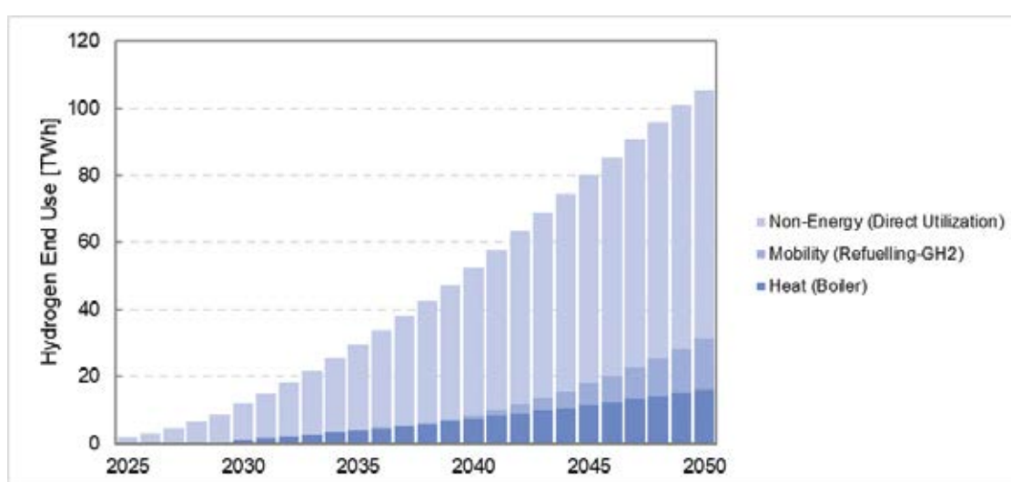
Figure 26: Hydrogen End Use Capacity by Technology Applications (BAU scenario)
