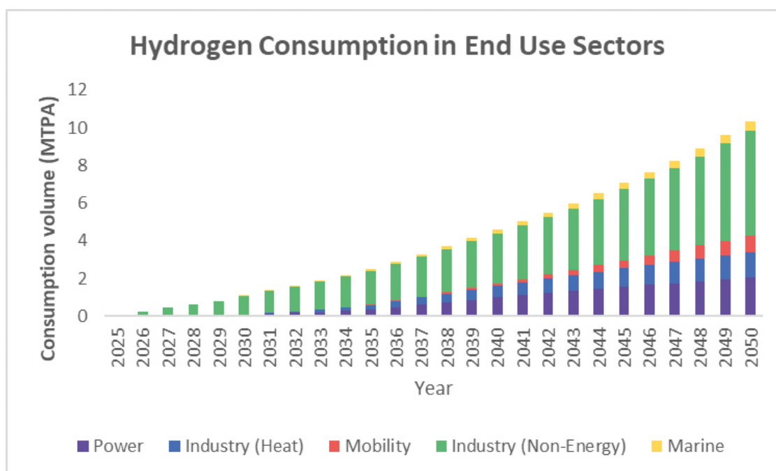
Figure 25: Hydrogen Consumption in End Use Sectors (Emission Driven Scenario)
