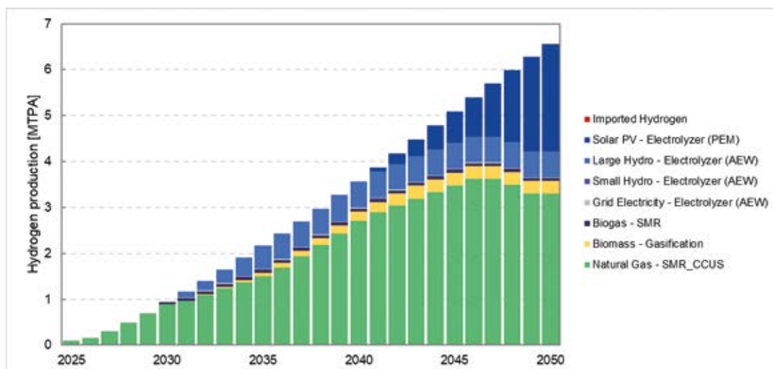
Figure 22: Hydrogen production (Business As Usual Scenario)
