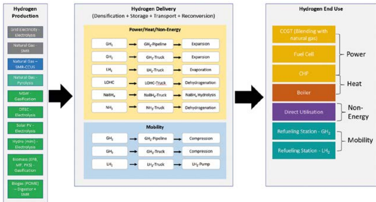
Figure 13: Technology across hydrogen economy value chain
