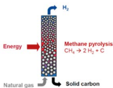
Figure 15: Methane pyrolysis for hydrogen and solid carbon production
