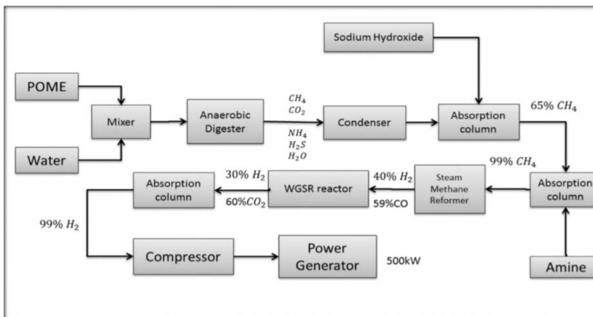
Figure A: Schematic diagram that shows pathway for Green Hydrogen production from Biogas (POME) – Digester + SMR
