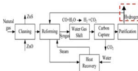
Figure 14: Hydrogen production from NG-SMR-CCUS
