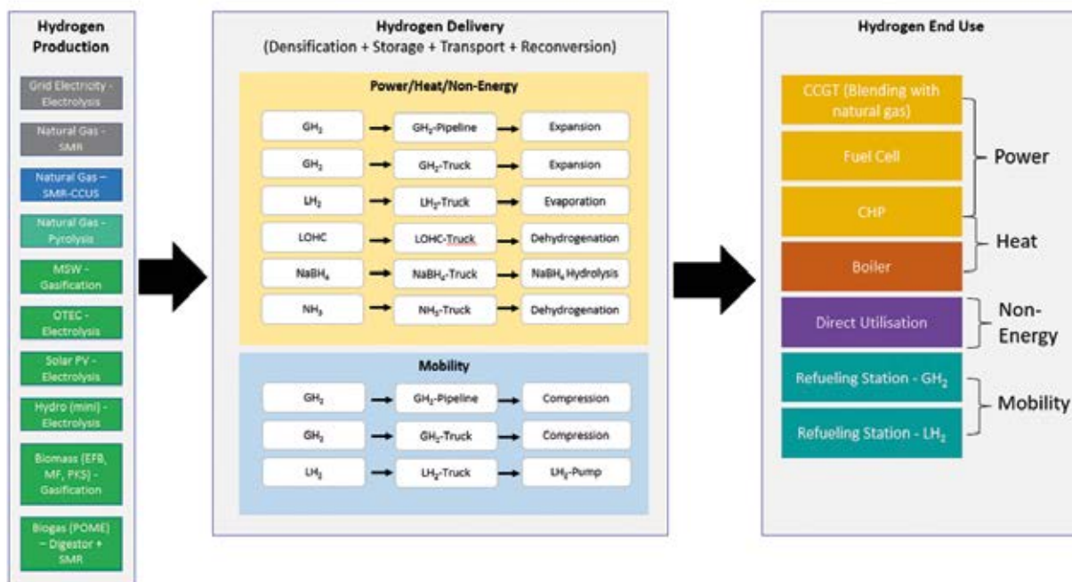
Figure 17: The HETR model in the form of modular components.
