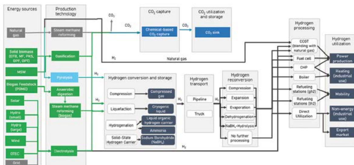
Figure 12: Hydrogen Supply Value Chain Superstructure Model
