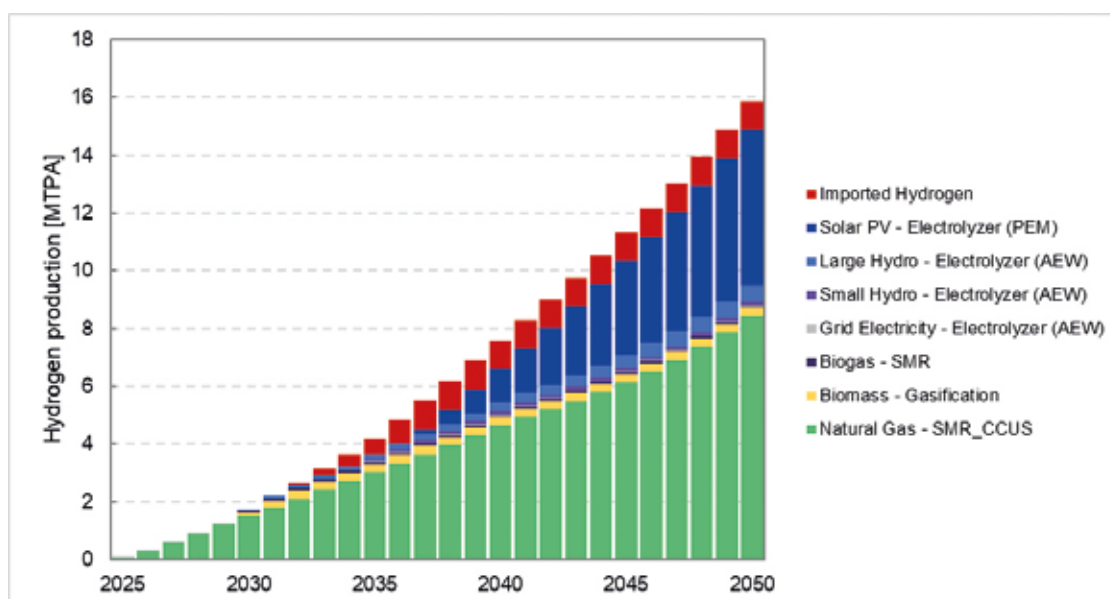
Figure 23: Hydrogen production (Emissions Driven Scenario)
