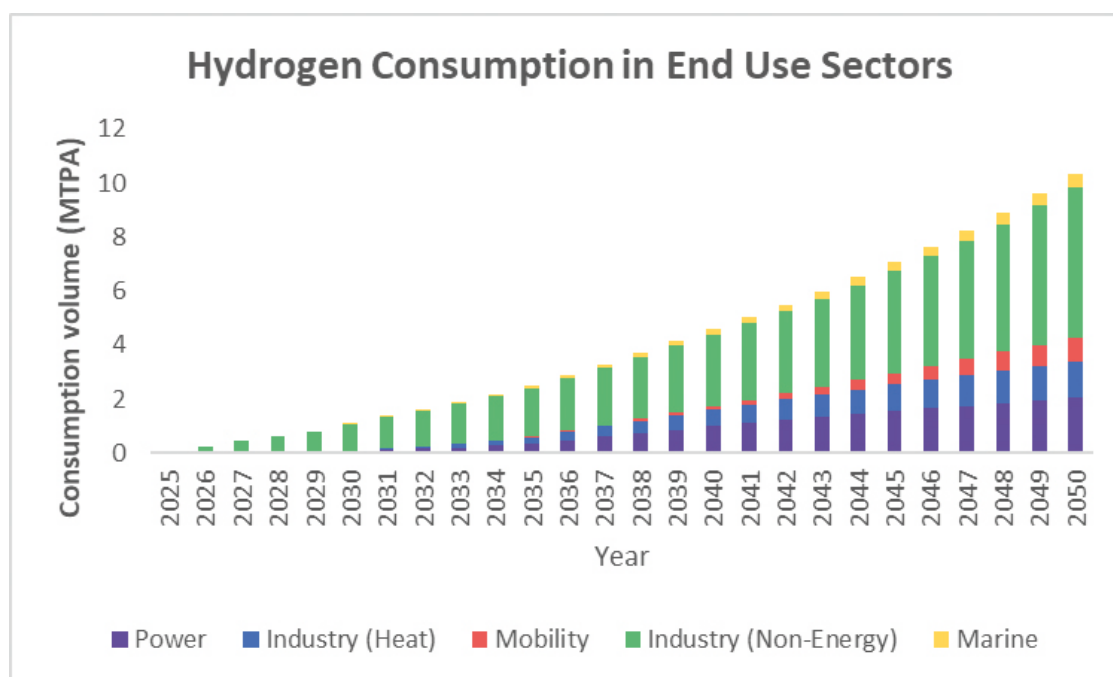
Figure 24: Hydrogen Consumption in End Use Sectors (BAU Scenario)
